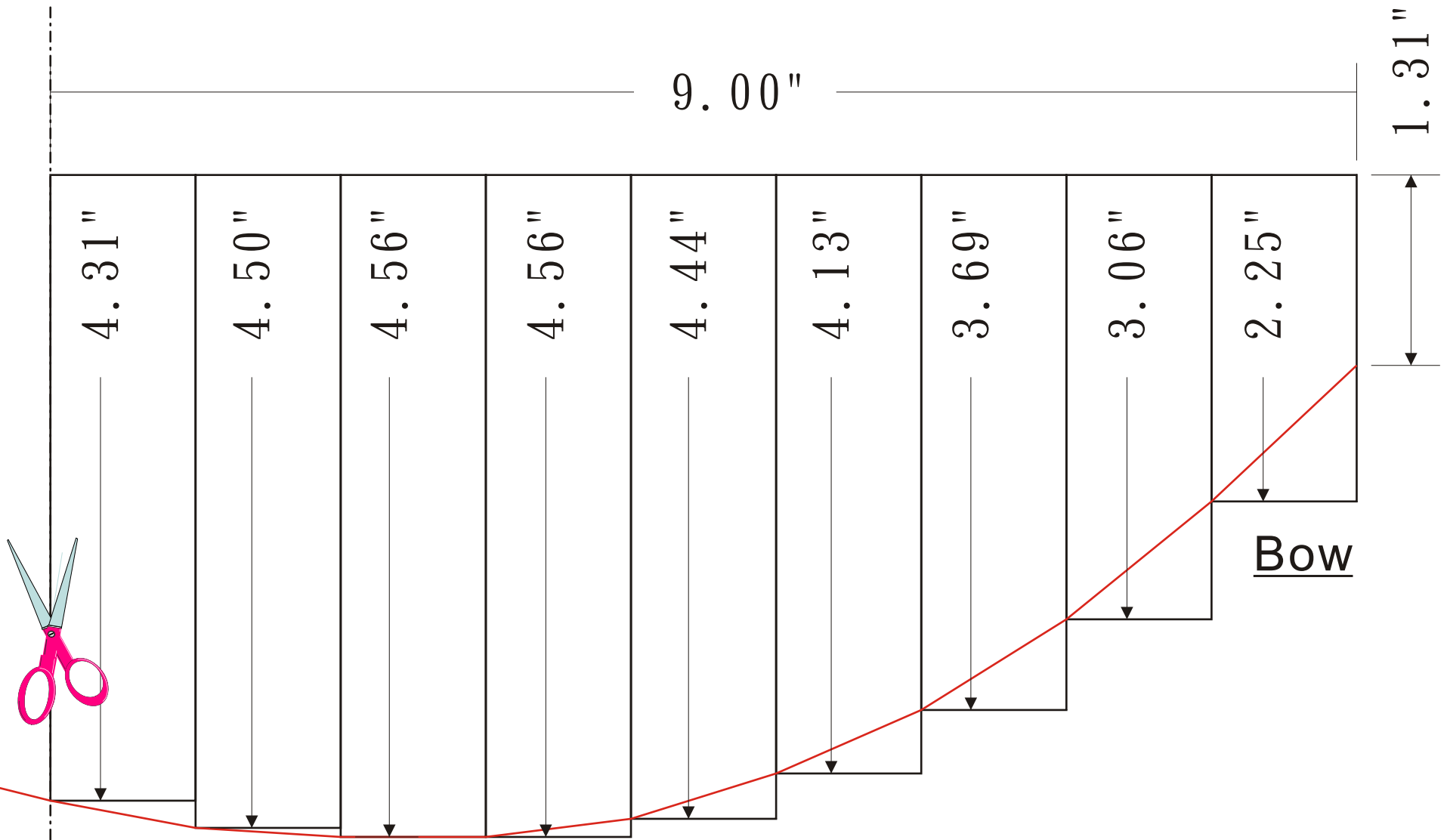
Springer Hull "Side Profile" Part B
