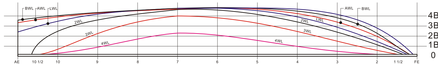
Sheer elevation
