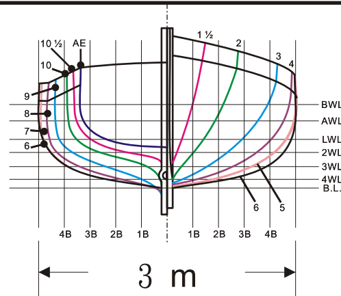
Waterline plan
